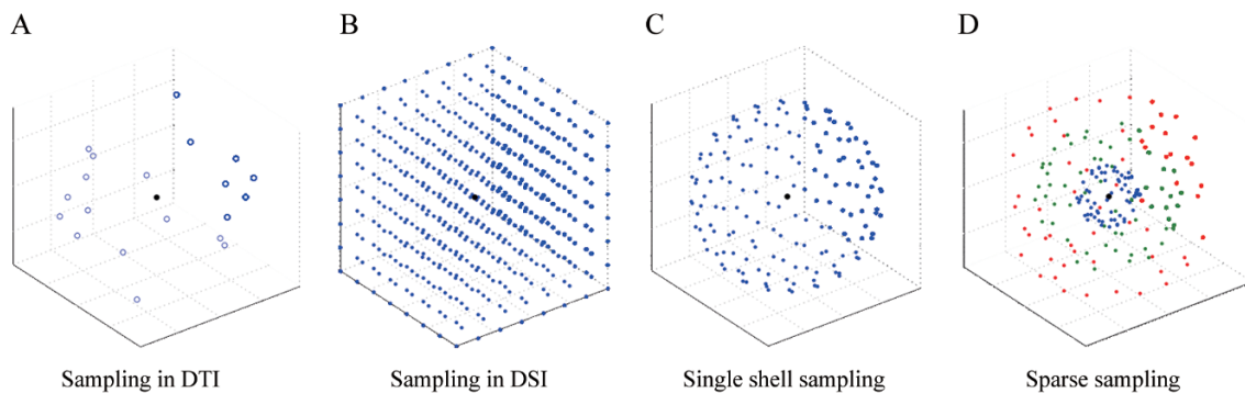
Fig. 3. Several kinds of sampling in q-space. The black dot in q = (0, 0, 0)T is the baseline image without a diffusion gradient. Note that although we showed sampling in R3, normally only samples in a half-space are used, e.g. q_z \geq 0 . A: Sampling used in DTI, normally <20 DWI images are used; B: Dense Cartesian sampling used in DSI; C: Single shell sampling; D: Sparse sampling.
