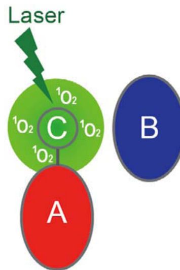
Fig. 1. Principles of CALI. Laser irradiation of a chromophore (C) generates ^1\text{O}_2 that inactivates an adjacent protein (A) without affecting other proteins (B).
