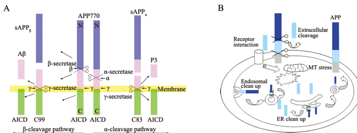
Fig. 1. APP processing and cleavage pathways. A: Two pathways of APP processing. In the \beta -cleavage pathway, APP is cleaved into sAPP_{\beta} (a secretory ectodomain) and C99 (a membrane-bound fragment). The C99 fragment is subsequently cleaved by \gamma -secretase to generate an intracellular domain of APP (AICD) and A\beta . In the \alpha -cleavage pathway, APP is cleaved into sAPP_{\alpha} (a secretory ectodomain) and C83 (a membrane-bound fragment). The C83 fragment is subsequently cleaved by \gamma -secretase to yield a 3-kDa fragment (P3) and AICD [1] . Cited from Huang et al. 2011, J Alzheimers Dis [1] . B: Newly-translated APP matures on the endoplasmic reticulum (ER) and Golgi apparatus. On one hand, mature APP is inserted into the cell surface by the delivery of secretory vesicles. On the other hand, either immature or mature APP might be cleaved at the ER and Golgi apparatus/trans-Golgi network. Cell surface APP is not only cleaved to generate A\beta on the cell surface, shedding A\beta into extracellular space, but is also endocytosed by the endosomal/lysosomal pathway and A\beta is shed into intracellular space. Both extracellular and intracellular A\beta might induce mitochondrial (MT) stress.
