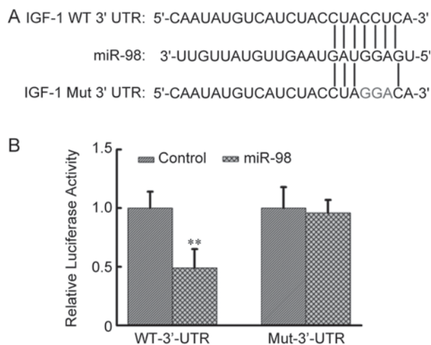
Fig. 2. IGF-1 is a direct target of miR-98. A: Schematic diagrams of binding of miR-98 with wide-type (WT) IGF-1 at the 3'-UTR, and the mutated (Mut) IGF-1 sequences. B: Dual-luciferase assays performed in HEK293 cells co-transfected with the reporter construct containing the 3'-UTR of the WT or mutated IGF-1 and the miR-98 overexpression plasmid or the control vector. Relative Renilla luciferase activity was normalized to firefly luciferase activity. Data are from 3 separate experiments (Student's t -test, ** P < 0.01 versus the IGF-1 WT 3'-UTR + control vector).
