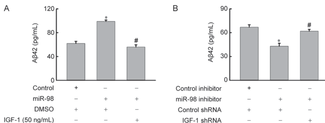
Fig. 4 MiR-98 increases A \beta production by targeting IGF-1. A: N2a/APP cells were transfected with miR-98 or the control vector and incubated with DMSO or 50 ng/mL IGF-1 for 48 h. Then the A \beta levels were measured using ELISA. B: N2a/APP cells were co-transfected with the miR-98 inhibitor or the control inhibitor and IGF-1 shRNA or the control shRNA for 48 h; the levels of A \beta were measured using ELISA. Data are from 3 separate experiments (Student's t -test, * P < 0.05 versus the first group, # P < 0.05 versus the second group).
