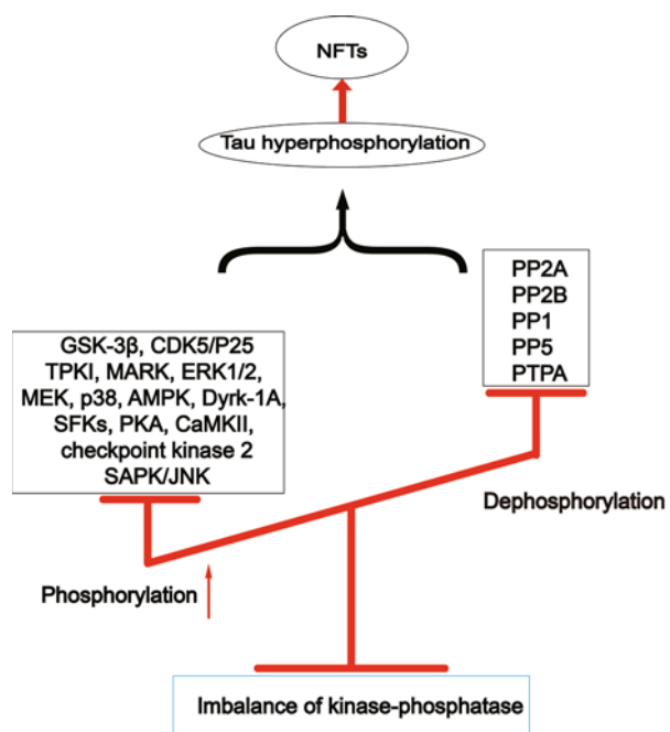
Fig. 3. Imbalance between tau-related kinases and phosphatases causes tau hyperphosphorylation. Hyperphosphorylation of tau is induced by the over-activation of kinases such as GSK-3 \beta and MARK, or the inactivation of phosphatases like PP2A, which further promotes the formation of neurofibrillary tangles.
