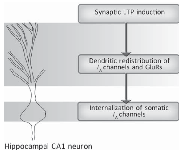
Fig. 1. I_A channel-mediated responses in dendrites and the soma of CA1 neurons after LTP induction. Synaptic LTP increases the local excitability of active synapses and dendritic branches via internalizing I_A channels from the membrane. Somatic excitability can be also influenced after LTP induction which enhances the intrinsic ability to fire action potentials through somatic I_A channel downregulation. Therefore, it seems reasonable that both synaptic and somatic regulation of I_A channels may be required to complete synaptic modification for the memory mechanism.
