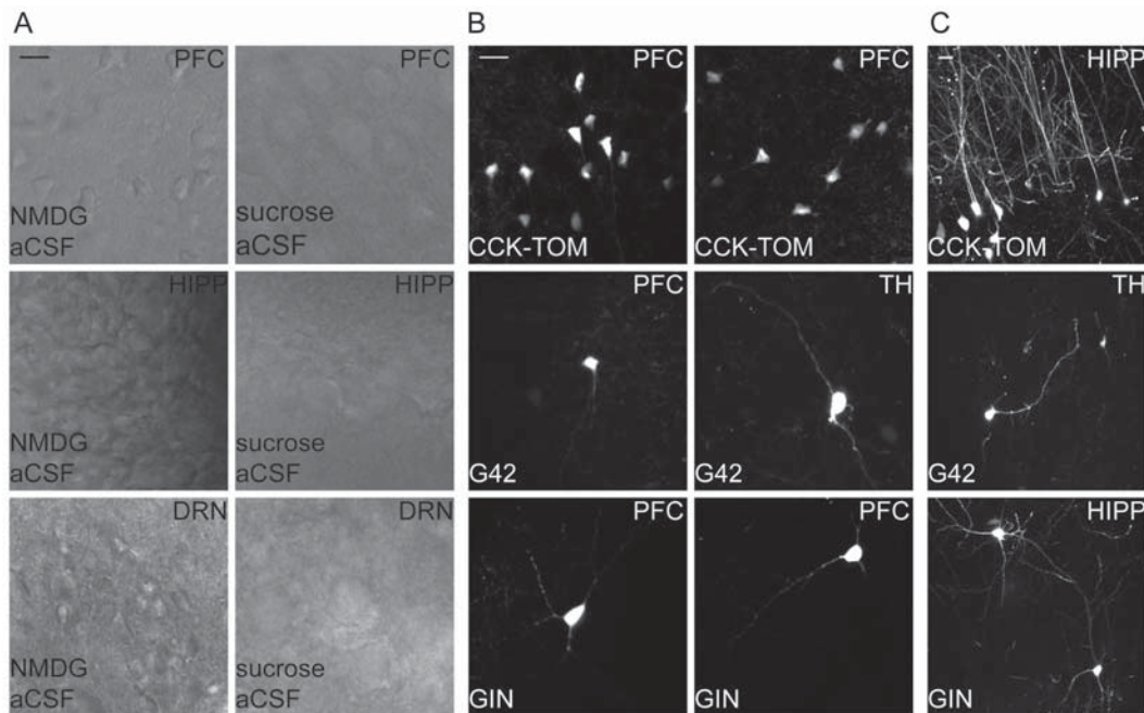
Fig. 1. Morphological preservation of neurons in brain slices. (A) Direct comparison of neurons (2–3 months old) from the prefrontal cortex (PFC), hippocampus (HIPP) and dorsal raphe nucleus (DRN) using the NMDG and sucrose aCSF methods. More neurons swell and die when prepared with sucrose aCSF. (B, C) Confocal microscopic images of neurons from the PFC, hippocampus, and thalamus (TH) from 3 transgenic mice (3–6 months old). Neurons display clear, healthy, and branched projections. Scale bars, 20 \mu m.
